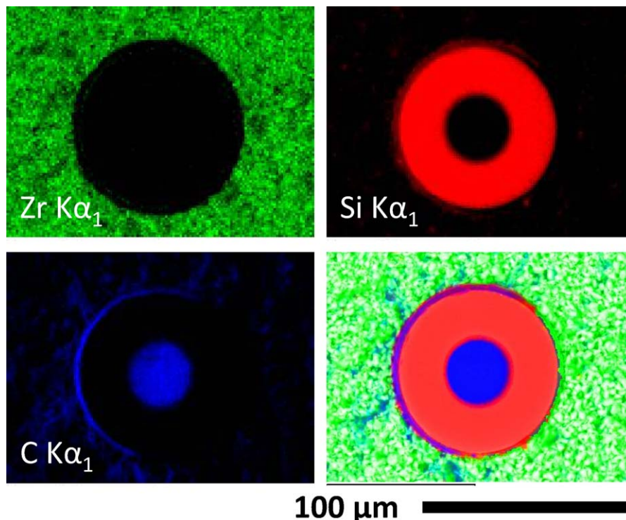
Fig. 3. EDS map of a section perpendicular to the fibers in the ZSS composite. Zr, Si and C elemental maps are included.
