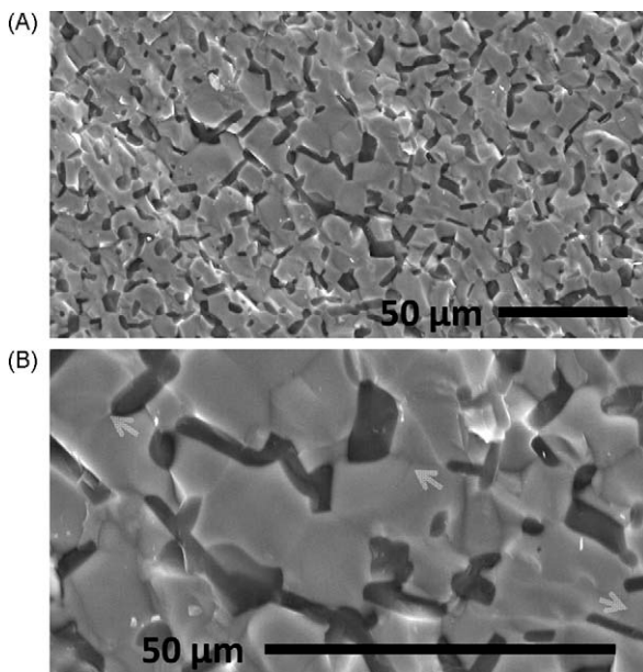
Fig. 5. Fracture surface in ZS after high strength compression tests. (A) General view showing grain pullout in SiC, and transgranular fracture in \text{ZrB}_2 . (B) Detail at higher magnification, showing intergranular small cracks.
