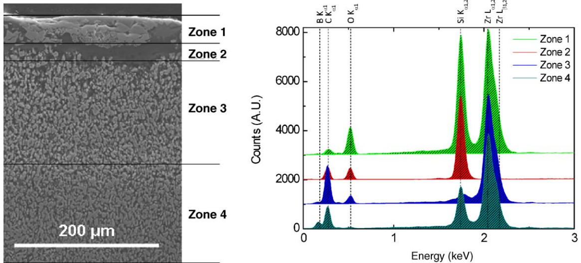
Fig. 11. (Left) Characteristic microstructure of ZSC samples after 24 h exposure to oxidizing atmosphere at 1400 °C. Several zones can be distinguished. (Right) Relevant EDS spectra obtained from the four zones depicted.
