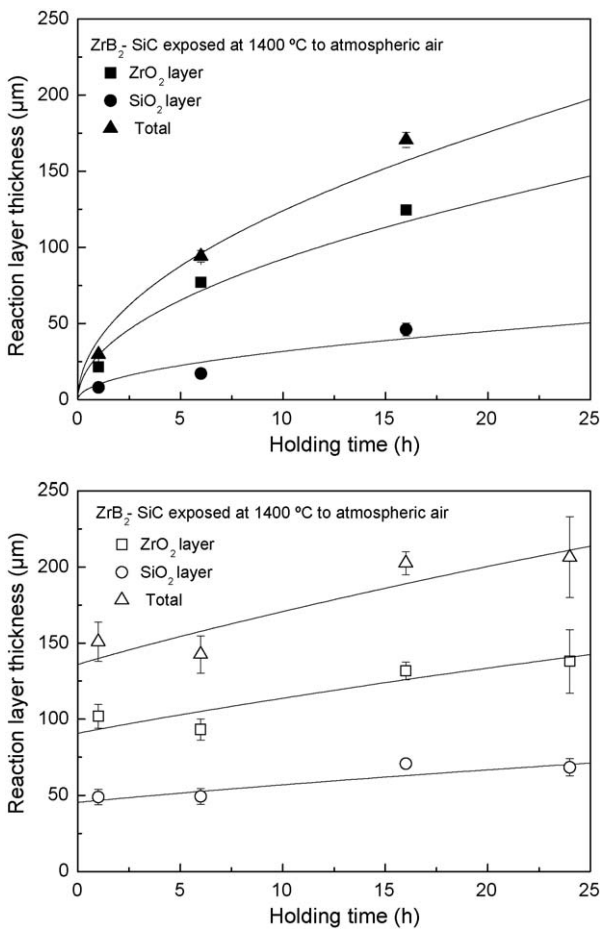
Fig. 12. Evolution of the oxide layer thickness with exposure time for ZS (top) and ZSC (bottom). The data has been fitted to a d \propto \sqrt{t + t_o} law which is characteristic of a diffusional process. For ZS, t_o \approx 0 .
