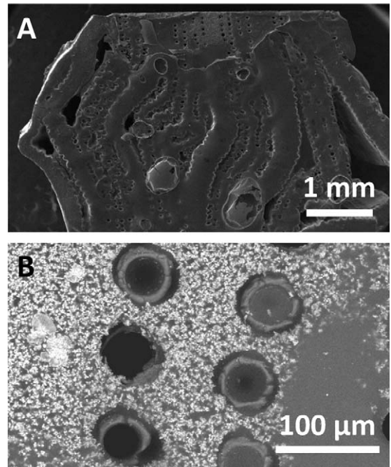
Fig. 8. Microstructure of ZSS after compression at 1550 °C in the trasversal direction. (A) General view (SE contrast) and (B) detail of the fibers (BSE contrast).
