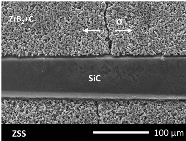
Fig. 2. Detail of the fiber and matrix in ZSS showing penny cracks in the matrix, perpendicular to the SiC fibers.
