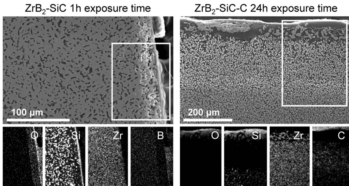
Fig. 10. EDS composition maps of ZS after oxidation for 1 h at 1400 °C (left) and of ZSC after oxidation for 24 h at 1400 °C.
