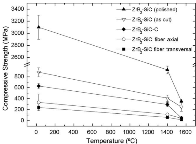
Fig. 7. Compressive strengths of ZS, ZSC, and ZSS as a function of temperature.
