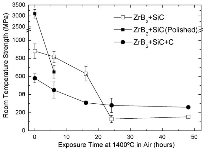
Fig. 9. ZS and ZSC compressive strength after oxidation in atmospheric air at 1400 °C.
